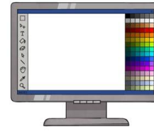
program
